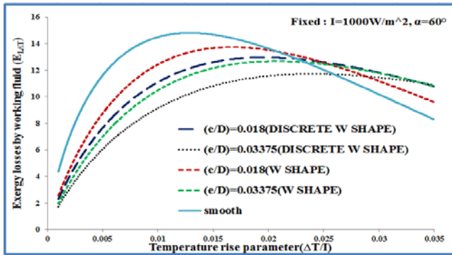
Fig.4. Variation of ( E_{L\Delta T} ) with temperature rise parameter for angle of attack ( \alpha ) of 60^\circ
