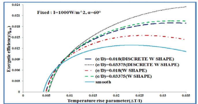
Fig.1. Variation of ( \eta_{exe} ) with temperature rise parameter for angle of attack ( \alpha ) of 60^\circ
