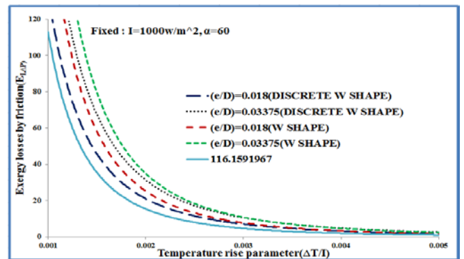
Fig.2. Variation of ( E_{LA} ) with temperature rise parameter for angle of attack ( \alpha ) of 60^\circ
